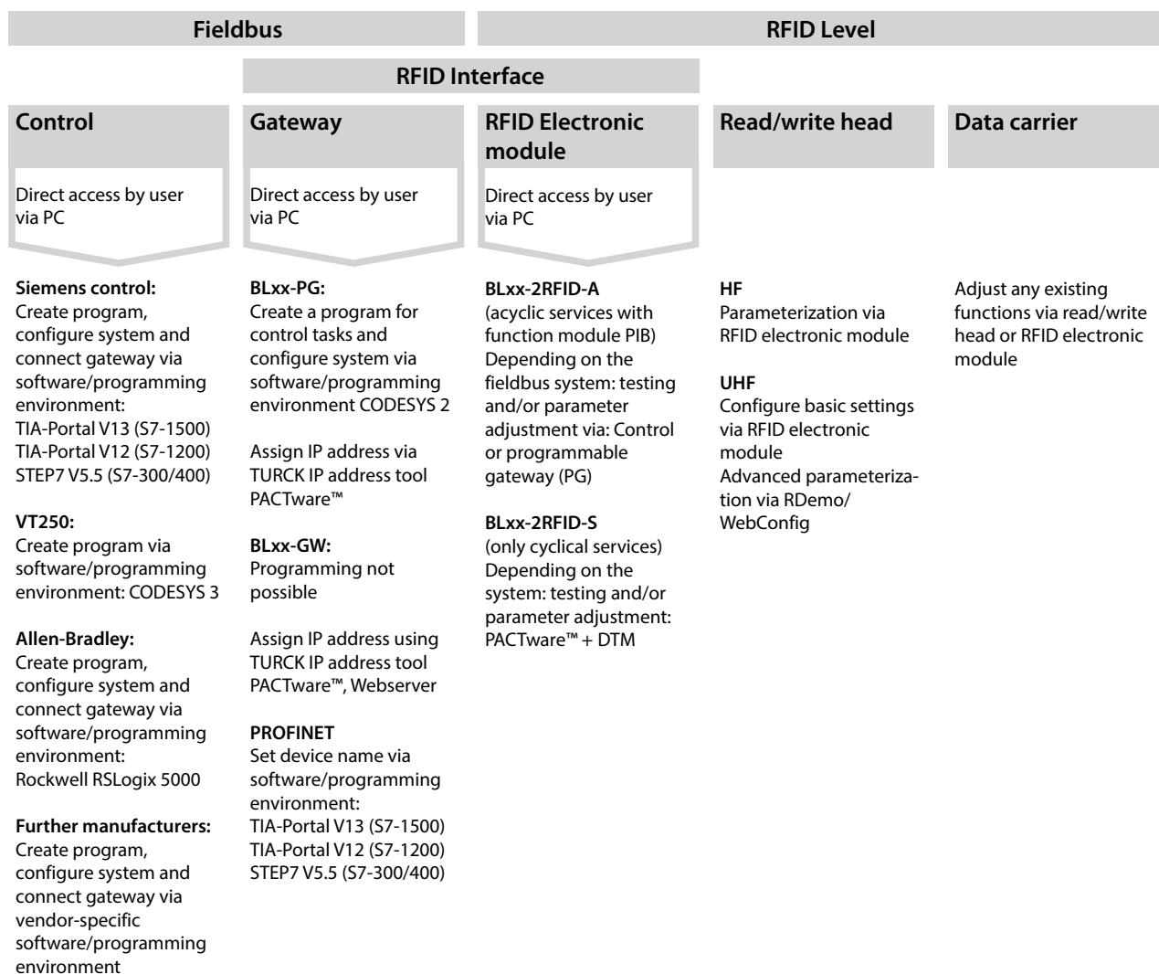
Fig. 2: Overview of BL ident® system levels and programming environments
