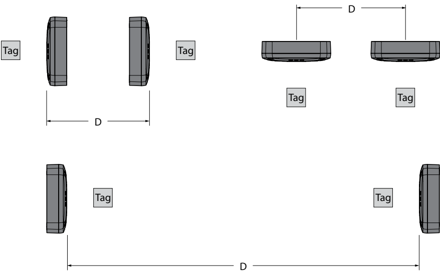
Fig. 32: Antenna alignment
